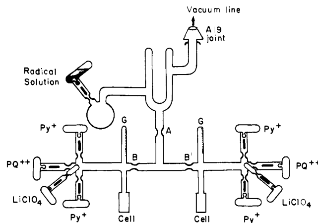
Figure 10. Measurement of association constant: Apparatus for the distillation of 1-methyl-2-(carbomethoxy)pyridinyl ( 2\cdot ) and the titration of solutions of the dimer (2-2) with 4^+\text{ClO}_4^- , followed by addition of \text{LiClO}_4 and then \text{PQ}^{2+}2\text{Cl}^- . The same apparatus is used to follow the reaction of 2^+\text{ClO}_4^- with 4\cdot . (See the description of the experiment in the caption for Figure 4.) The apparatus consists of two independent sides, allowing a test of reproducibility. After introduction of a radical solution and sealing off at A (see caption for Figure 9), the radical solution is poured around both sections of the manifold before sealing off at B or B'. \text{Py}^+ may be either 4^+ or 2^+ , depending upon the experiment. \text{PQ}^{2+} is paraquat dichloride. G is a graduated tube for measurement of the volume of the solution.
