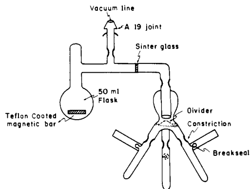
Figure 8. Apparatus for the preparation and distribution of solutions of stable pyridinyl radicals or pyridinyl radical dimers.
