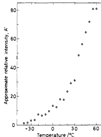
Figure 12. Plot of relative line intensity vs. temperature in the EPR spectrum of 1-methyl-2-(carbomethoxy)pyridinyl radical ( 2 ) in CH 3 CN, C 0 (dimer = 2.11 × 10 -3 M. The units of A' are arbitrary.
