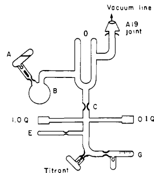
Figure 9. Apparatus for titration of pyridinyl radicals or radical dimers after distillation. A sample tube for ESR is also attached. The radical solution (cf. Figure 8) in the breakseal tube A is transferred to the distilling flask B, the solvent distilled into a receiver on the vacuum line, liquid \text{N}_2 poured into the Dewar, and the radical gently warmed [ 25 – 50^\circ\text{C} is normally sufficient for 2\cdot or (\text{CH}_3\text{CO})_2 ]. A blue or green solid condensate collects on the Dewar. Pure \text{CH}_3\text{CN} is distilled from the line onto the Dewar, the liquid \text{N}_2 removed, and the solution allowed to flow into the manifold below. The manifold is sealed off at the constriction C. Some solution is poured into the ESR and tube E, which is then sealed off. After volume measurement (graduated tube G), the radical (or radical dimer) solution is mixed with the titrant, and the spectrum of the solution is taken. Two cells l = 1.0 cm and l = 0.1 cm ensure that the OD will be in an accessible range.
